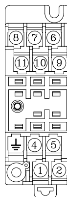
Pin Location
